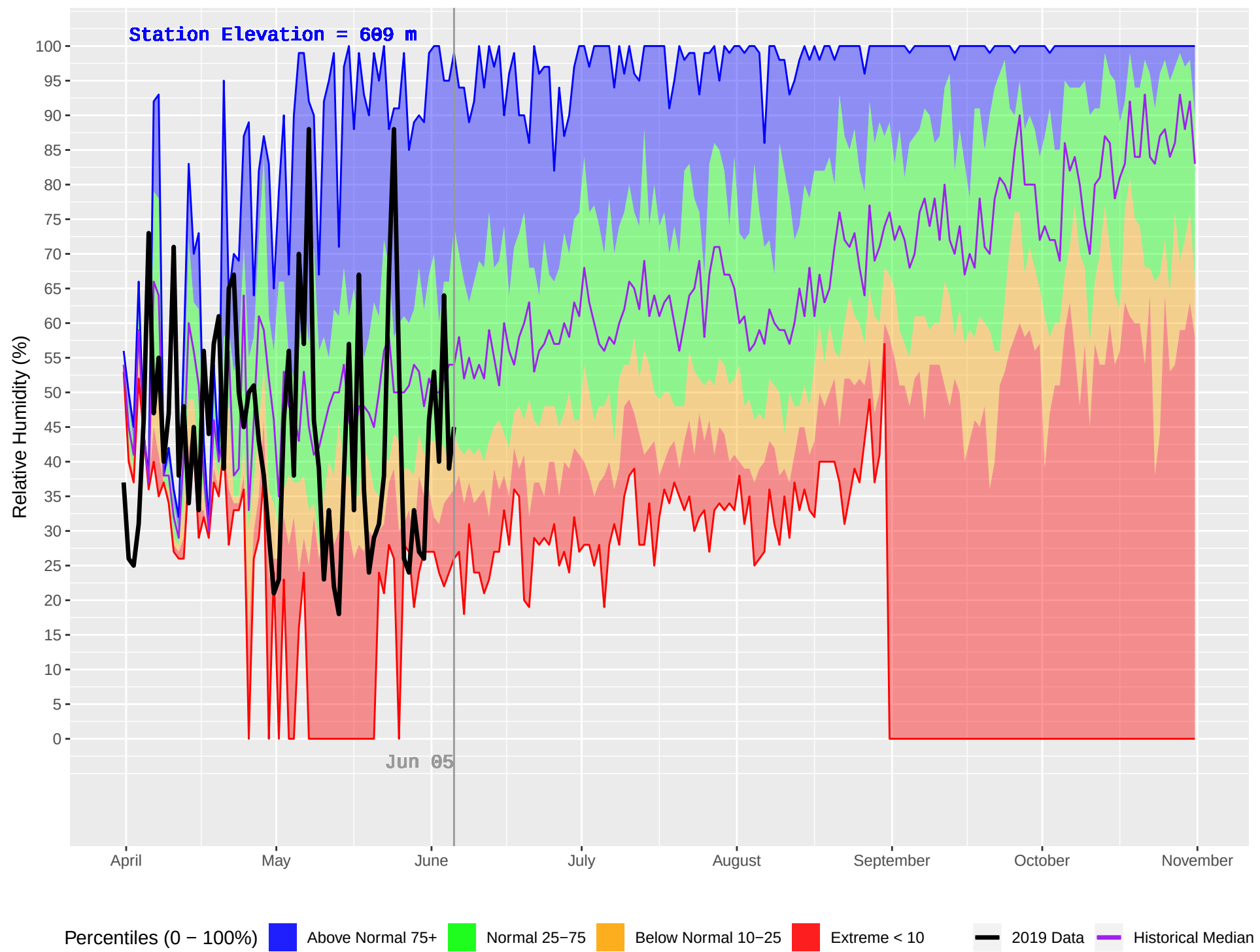
BOB QUINN LAKE (113) : Historical (1984–2018) and Current (2019) Daily Relative Humidity
