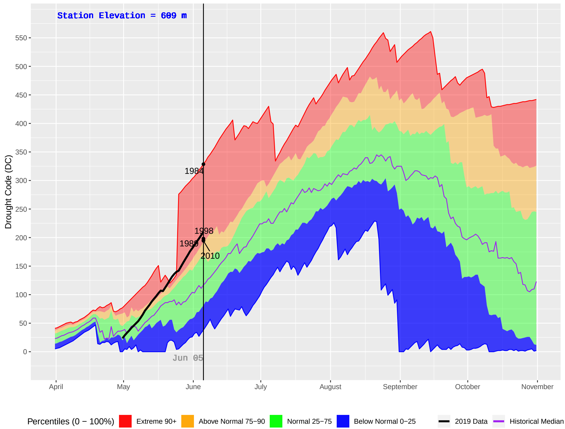
BOB QUINN LAKE (113) : Historical (1984–2018) and Current (2019) Daily Drought Code (DC)
