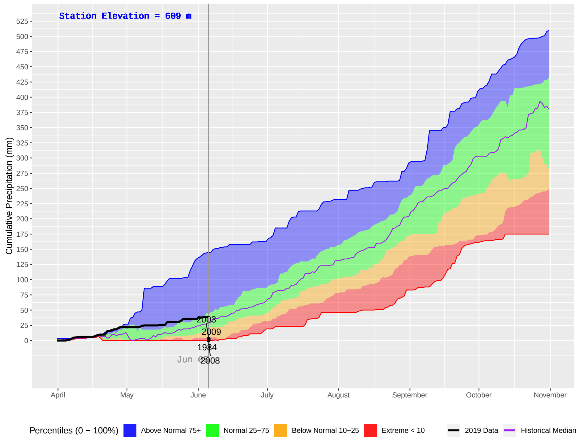
BOB QUINN LAKE (113) : Historical (1984–2018), Current (2019) Daily Cumulative Precipitation
