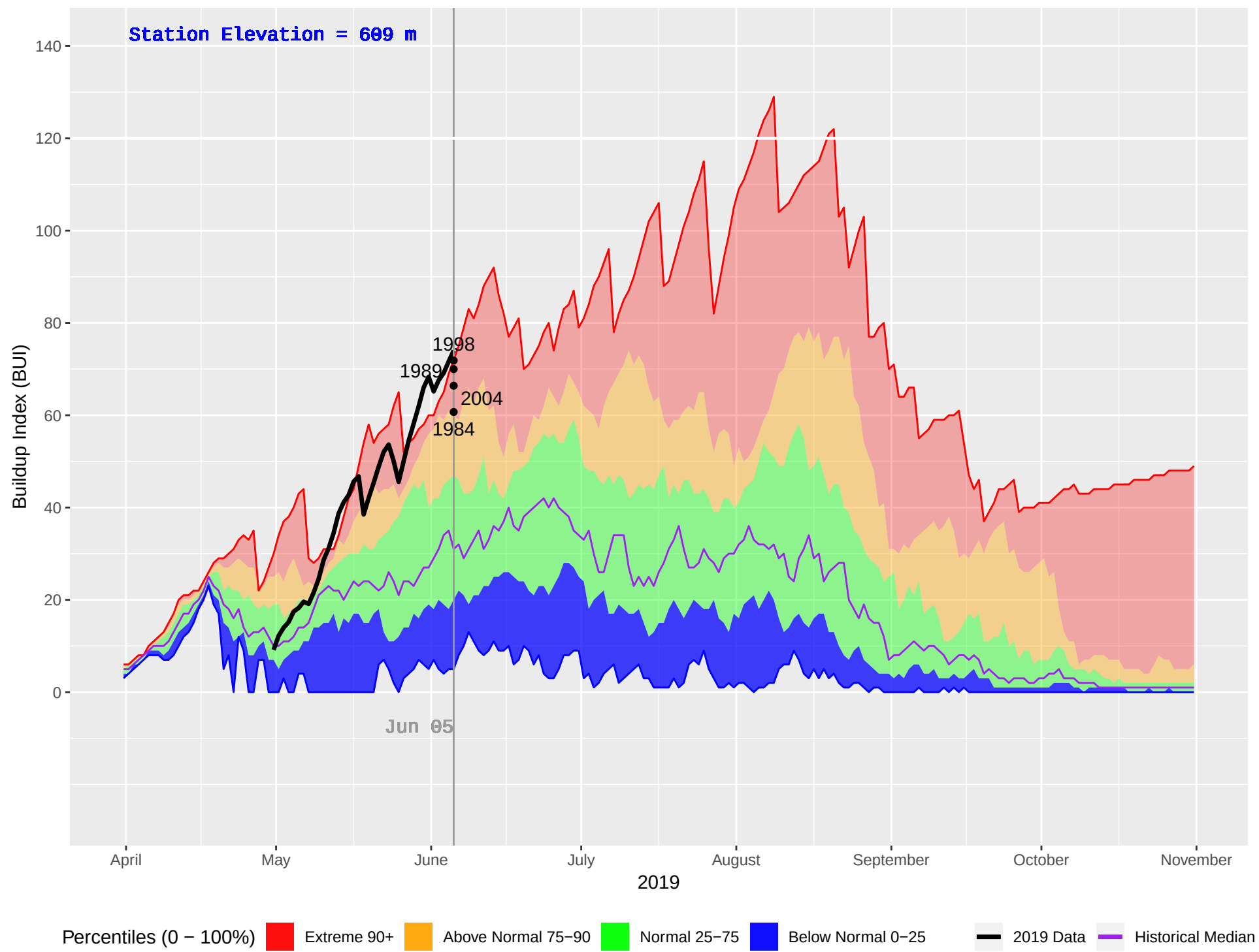
BOB QUINN LAKE (113) : Historical (1984–2018), Current (2019) Daily Buildup Index (BUI)
