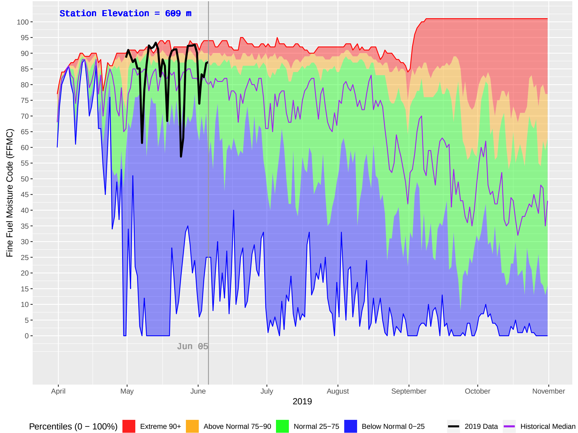
BOB QUINN LAKE (113) : Historical (1984–2018) and Current (2019) Daily Fine Fuel Moisture Code (FFMC)
