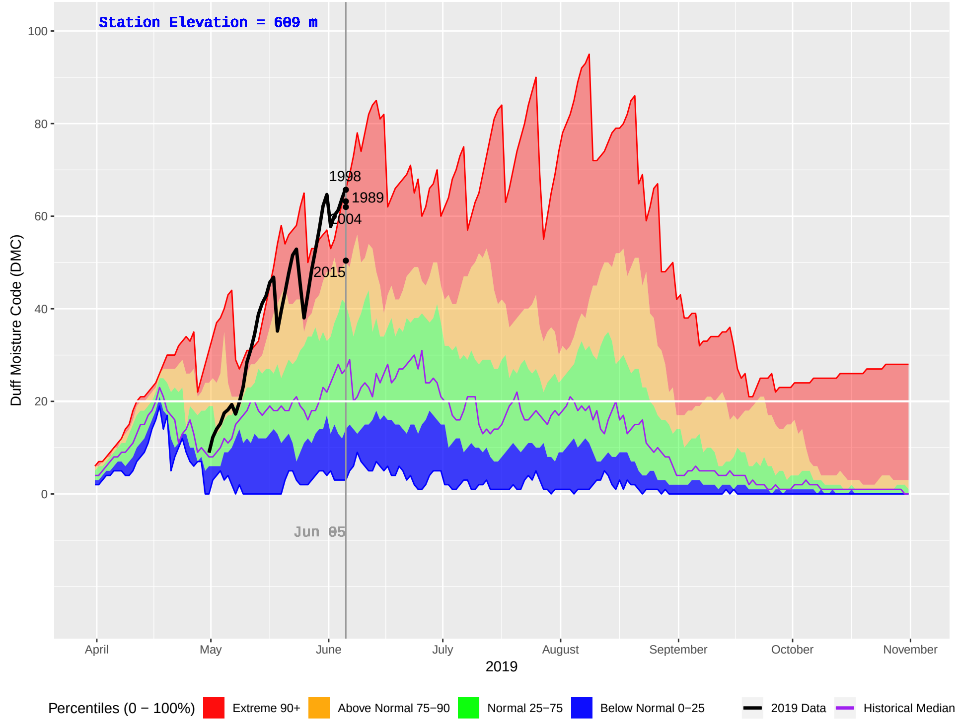
BOB QUINN LAKE (113) : Historical (1984–2018), Current (2019) Daily Duff Moisture Code (DMC)
